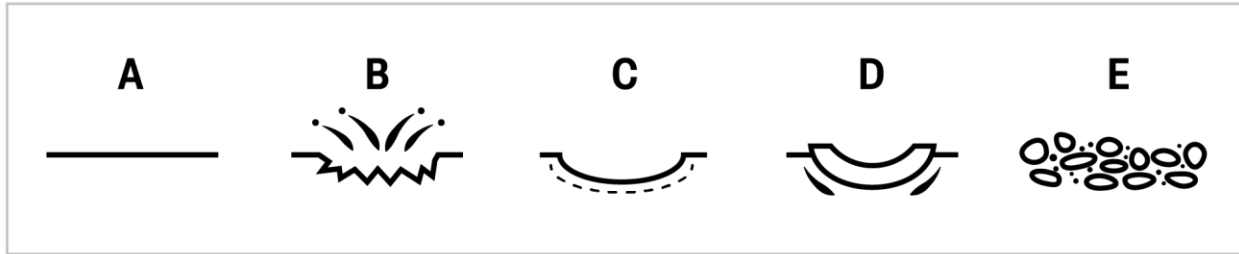
Figure 2. Figure 2 from Williamson and Kuhn, 1987 illustrates rock strength based on hammer impacts. Original figure caption: Reaction to impact of a ballpeen hammer. A) Rebound quality, no reaction; B) Pit quality, rough pit; C) Dent quality, smooth depression; D) Crater quality, depression with upthrust material around perimeter; E) Moldable quality, crumbles with finger pressure.
